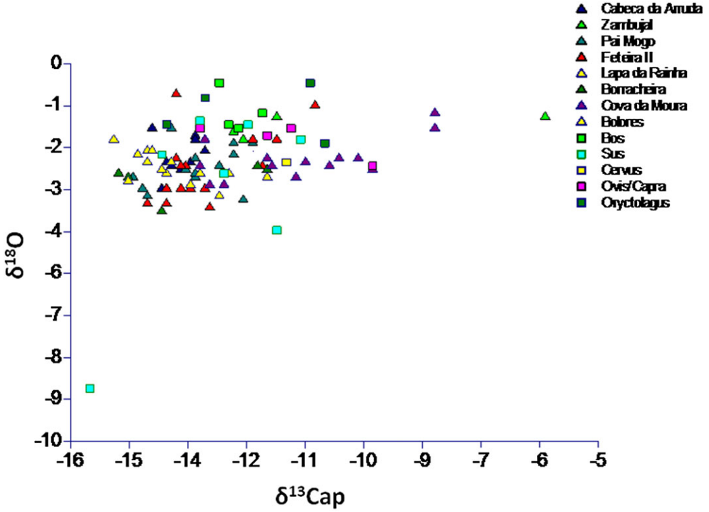
Figure 3 Scatter plots of apatite values for humans and fauna.
